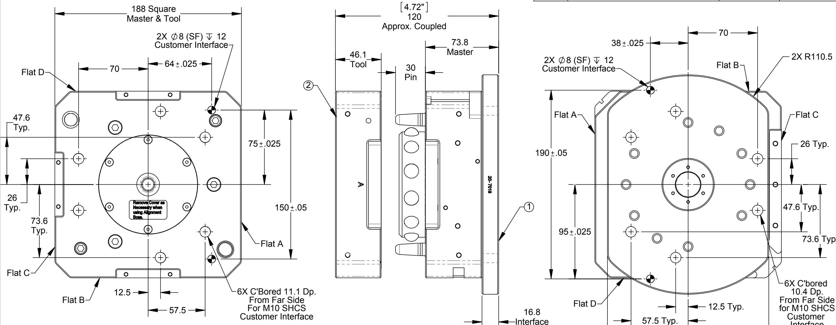
Tool Side (Projection Only)
