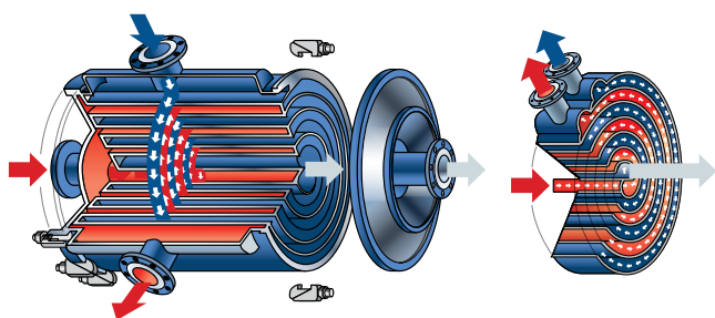
Horizontal configuration
