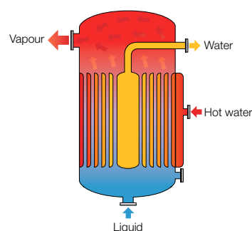
Evaporator/re-boiler
