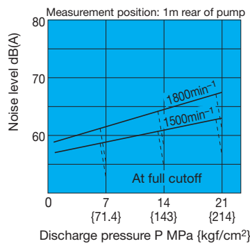
Noise Characteristics
