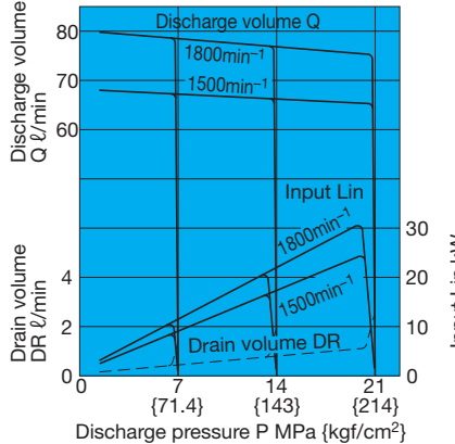
Pressure - Discharge Volume Characteristics
