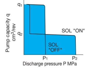
P-Q Characteristics
