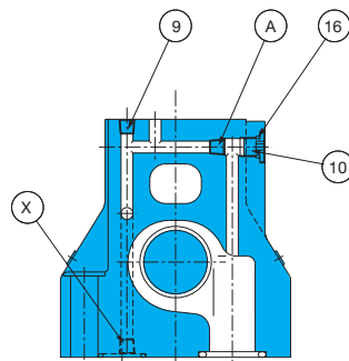
Cross-sectional P-P
