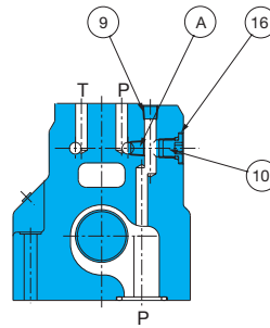
Cross-sectional P-P
