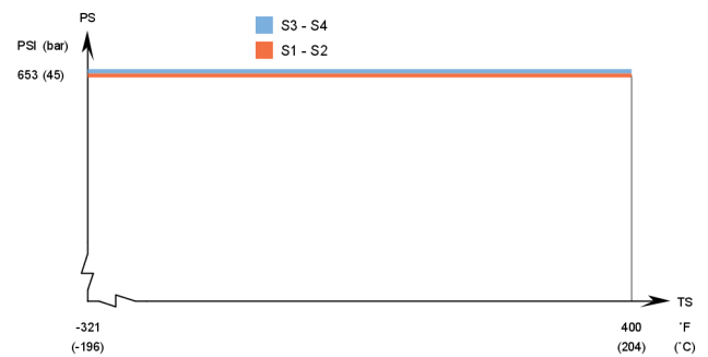
AlfaNova HP 76 – UL approval pressure/temperature graph 1)
