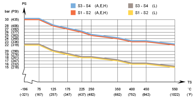
AlfaNova 76 – PED approval pressure/temperature graph 1)
