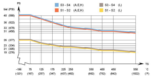
AlfaNova HP 76 – PED approval pressure/temperature graph 1)
