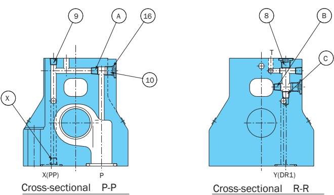
Changing the Pilot and Drain Connections
