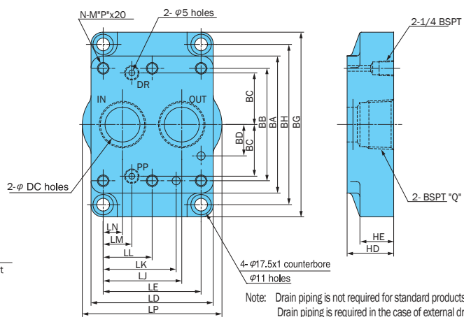
Sub Plate MCP**-**-20
