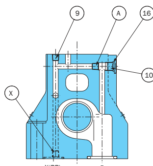
Cross-sectional P-P
