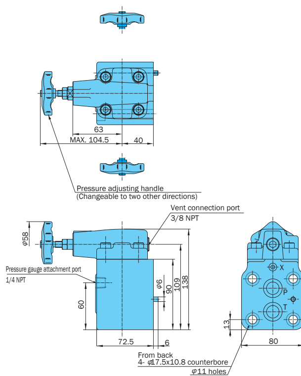
R-G**-*-20 (Gasket Mounting)
