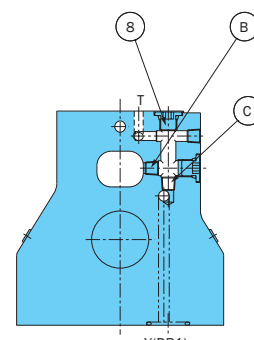
Cross-sectional R-R
