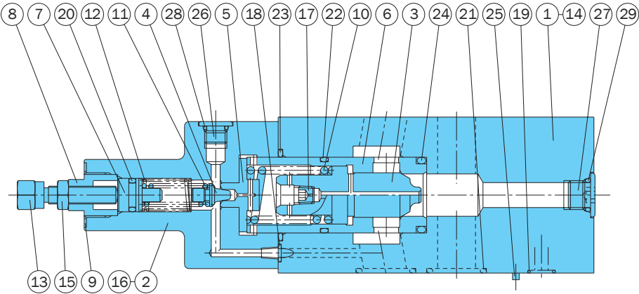
Seal Part List (Kit Model Number BRKS-04RP)
