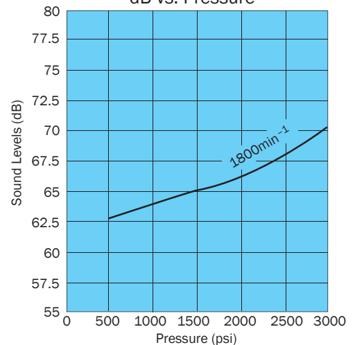
dB vs. Pressure
