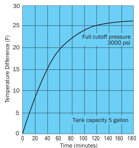
Oil Temperature Difference vs. Time
