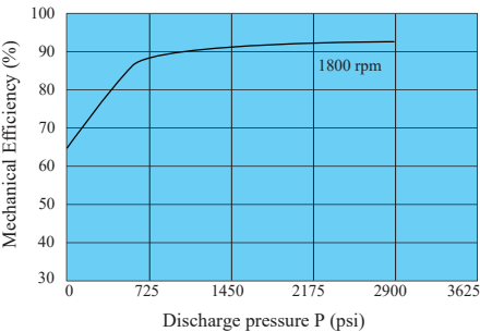
Mechanical Efficiency
