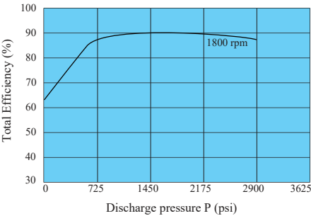
Total Efficiency
