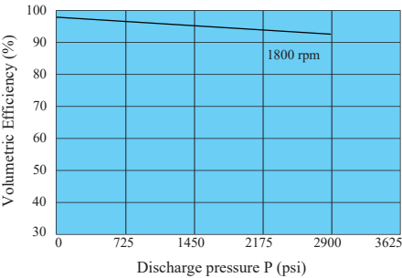
Volumetric Efficiency
