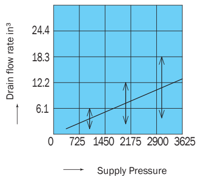
OGH-G04-*3-10
