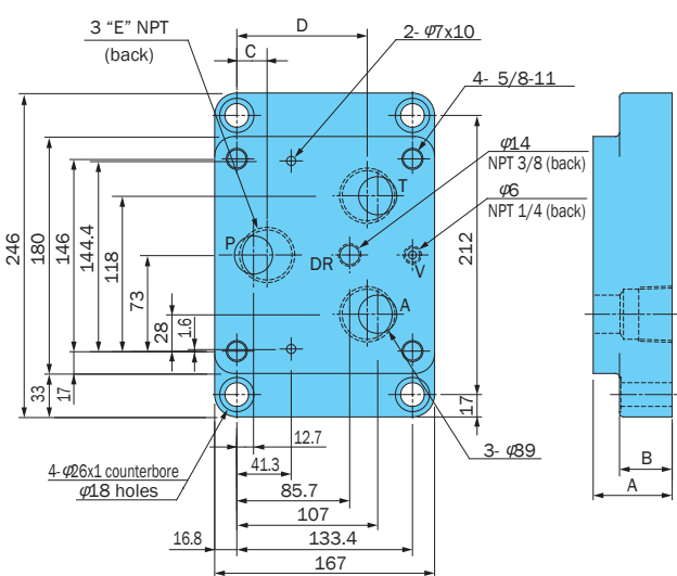
MSR-06*-E10
