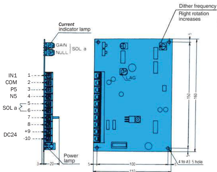
EBA-PD1-N-D2-10
