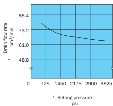
OGH-G04-P3-10
