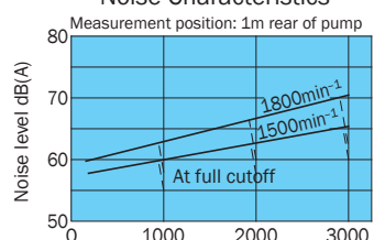
Noise Characteristics
