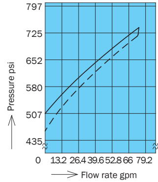
(C)Q-*10-2C-21
