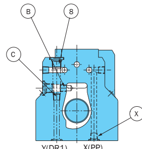
Cross-sectional R-R
