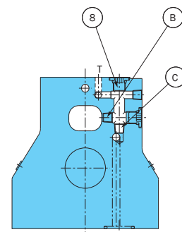
Cross-sectional R-R
