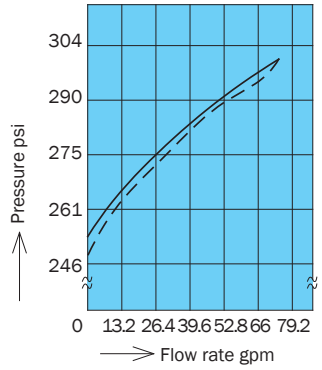
(C)Q-*10-2B-21
