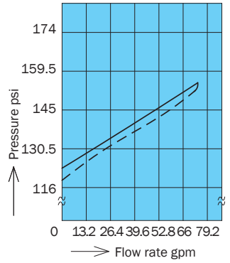
(C)Q-*10-2A-21
