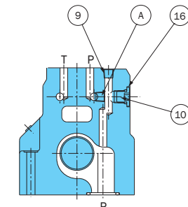
Cross-sectional P-P
