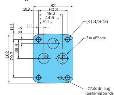
Mounting Gasket Dimensions EGB-G06-*-11
