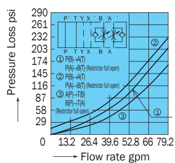
OYH-G04-W-Y-10 (OYH-G04-W-X-10)
