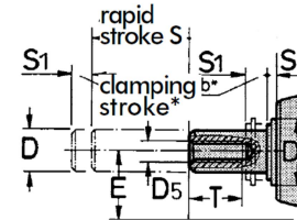
Shaft detail
