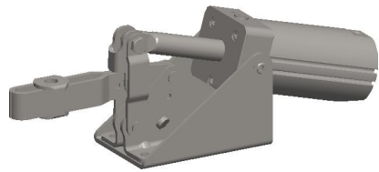
CLOSED POSITION
