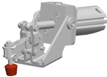
CLOSED POSITION
