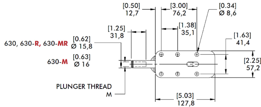
CLOSED POSITION
