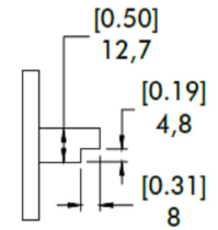
Arm Configuration
