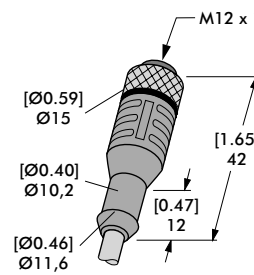
Straight: 8EL-002-1
