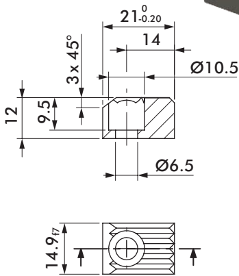
Steel Teeth Serrated Part # 8JZ-014-3
