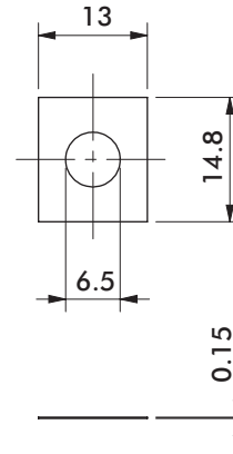
Shims Shims for Gripper Teeth Part # 8SB-003-1
