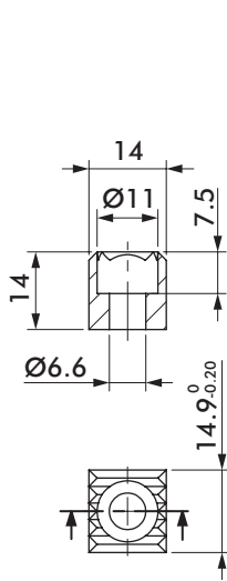
Steel Teeth Serrated Part # 8JZ-001-1
