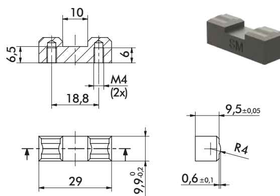
Hardened Steel Teeth Part # 8JZ-038-1 Crown Upper
