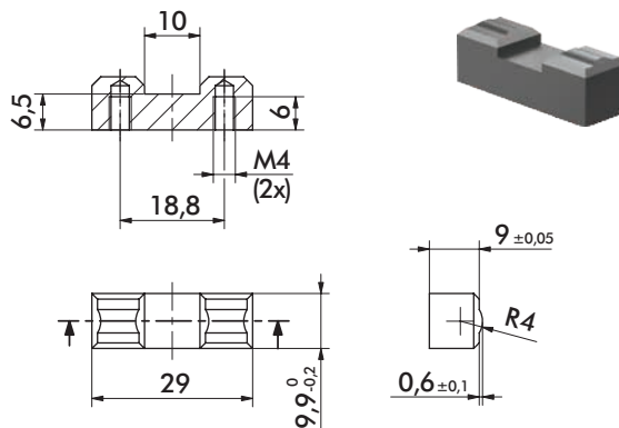
Hardened Steel Teeth Part # 8JZ-040-1 Crown Upper
