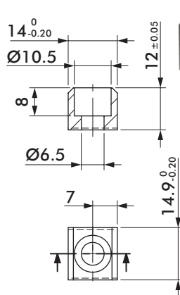
Steel Teeth Flat Part # 8JZ-050-1
