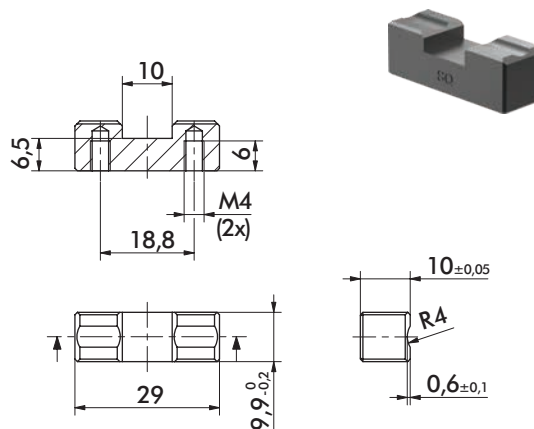
Hardened Steel Teeth Part # 8JZ-051-1 Crown Lower
