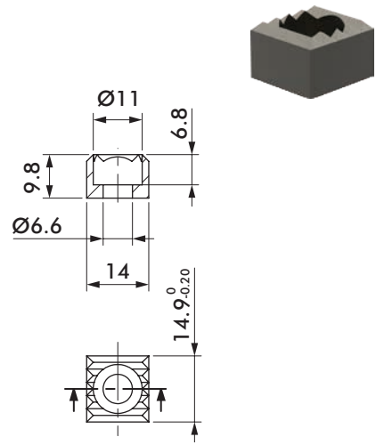
Steel Teeth Serrated Part # 8JZ-003-1
