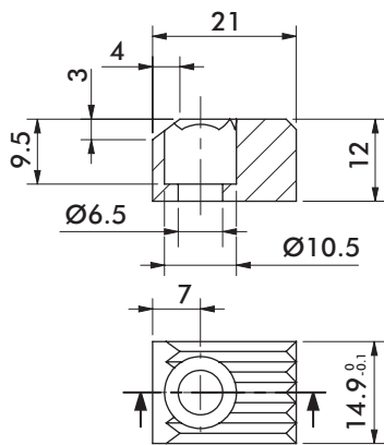
Steel Teeth High Temperature, Serrated Part # 8JZ-094-1
