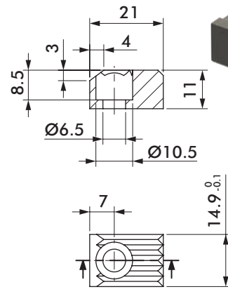
Steel Teeth Serrated Part # 8JZ-066-1
