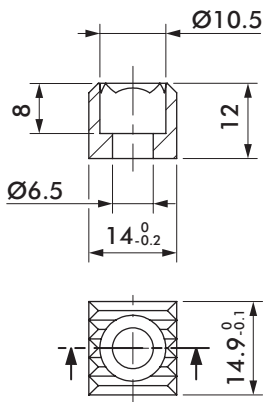
Steel Teeth Serrated Part # 8JZ-043-1
