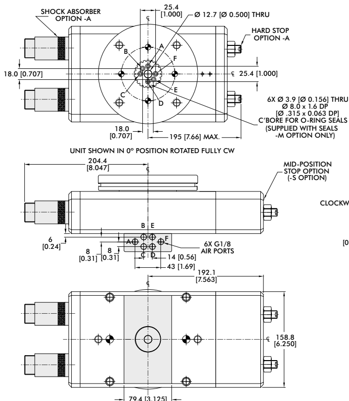
MID-POSITION STOP VIEW SHOWN
