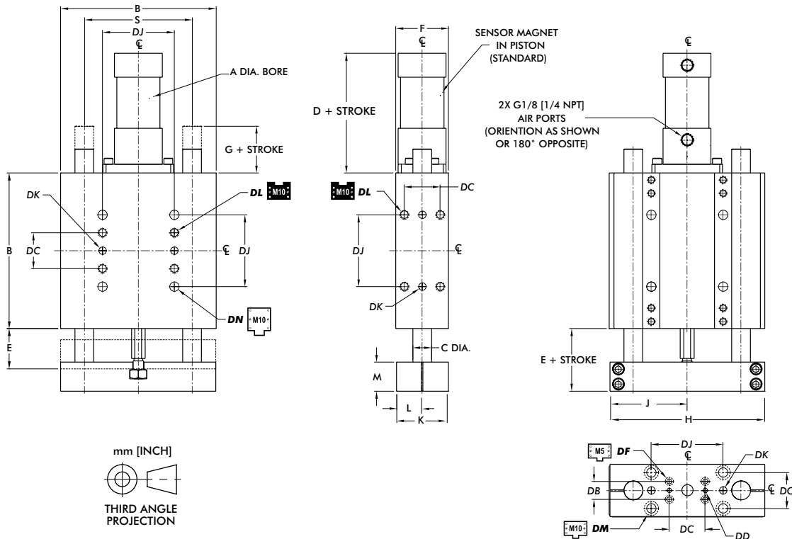
DIRECTCONNECT™ Mounting Pattern Dimensions (all sizes)
