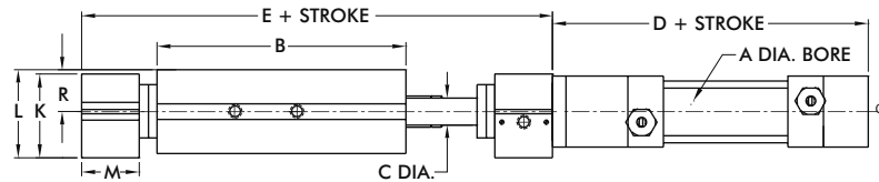
DIRECTCONNECT™ Mounting Pattern Dimensions (all sizes)
