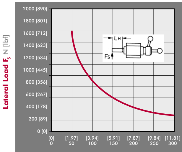
Allowable side load F_s depending on the stroke length L_H
