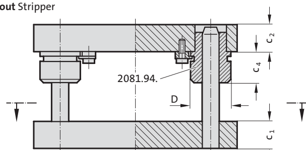
with Stripper
