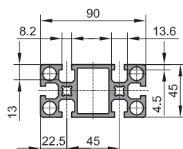
Profile cross-section
